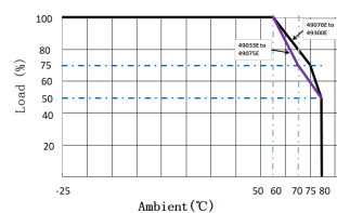
Power Derating Curve
